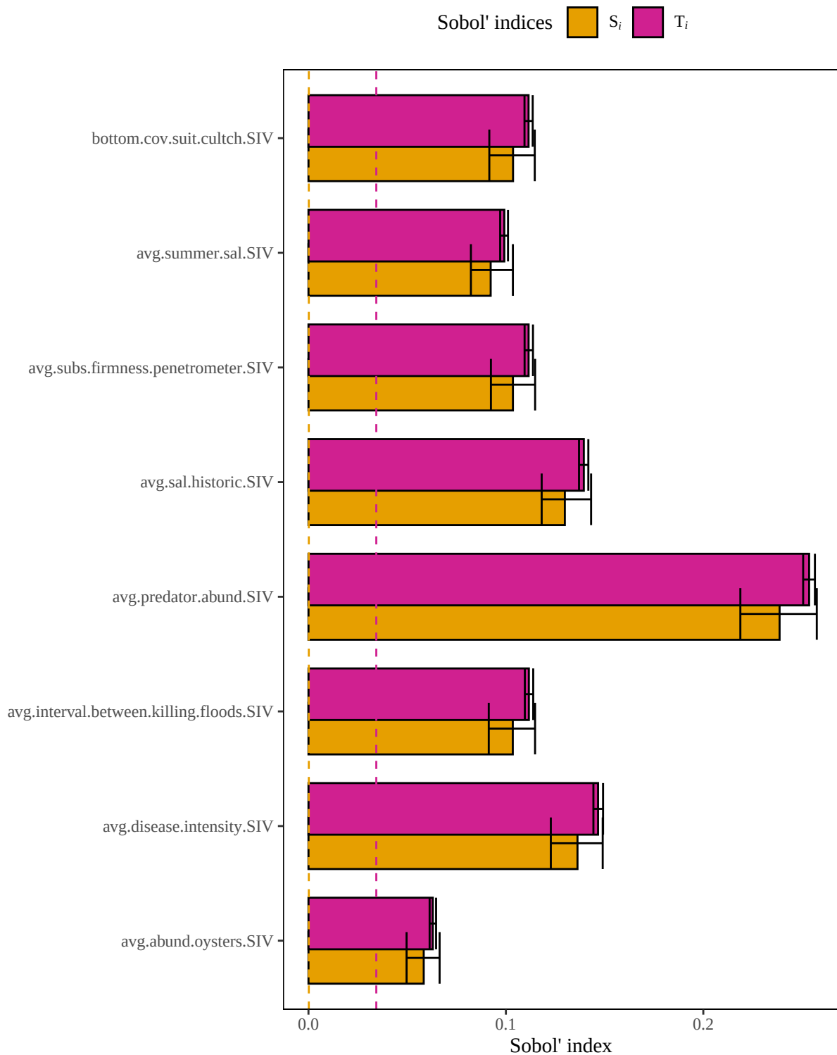
Figure 5. Results of a sensitivity analysis for the americanoysterGulfofMexModifier model based on a geometric mean structure. Dashed lines represent baseline numerical approximation error for S_i and T_i ( i.e. , dummy variables).
